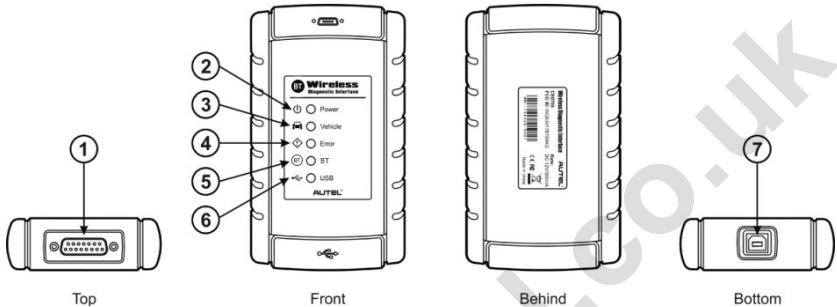
Figure 2-5 Wireless Diagnostic Interface
